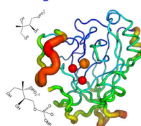
Design of new acaricides
