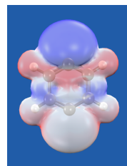
Reactive singlet geminal of para-benzyne
